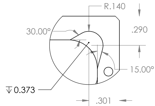
DETAIL G SCALE 2 : 1
